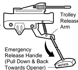
LOCKOUT POSITION
