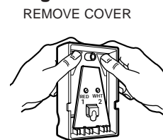
Figure 4 REMOVE COVER
